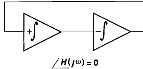
Fig. 6. Two-integrator oscillator.
