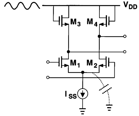
Fig. 17. Substrate and supply noise in gain stage.
