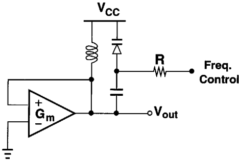
Fig. 4. LC oscillator.
