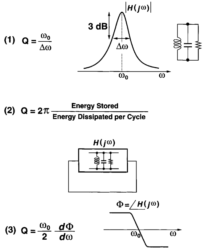
Fig. 5. Common definitions of Q .
