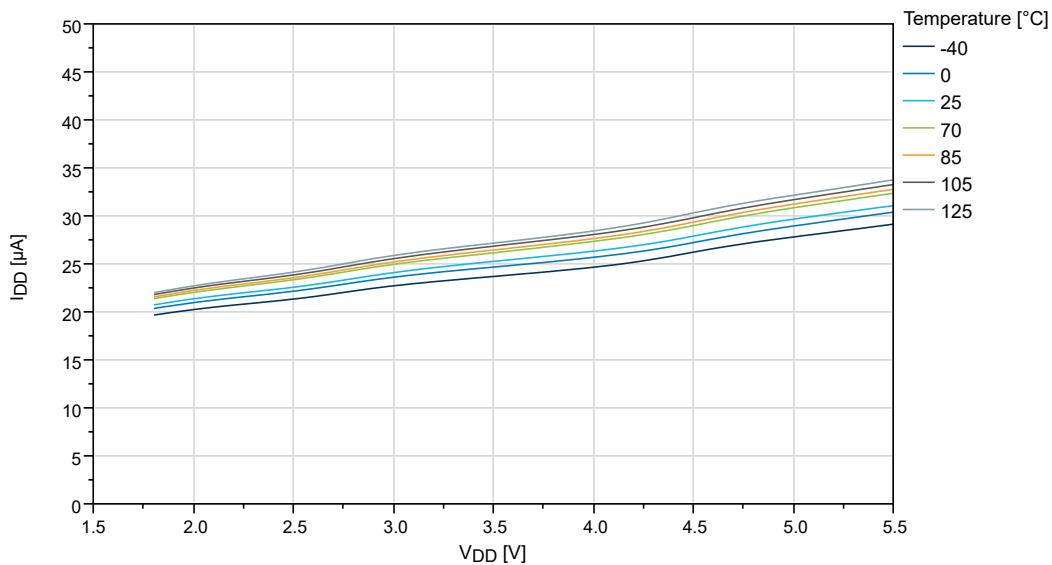
Figure 34-20. BOD Current vs. V_{DD} (Continuous Mode enabled)
