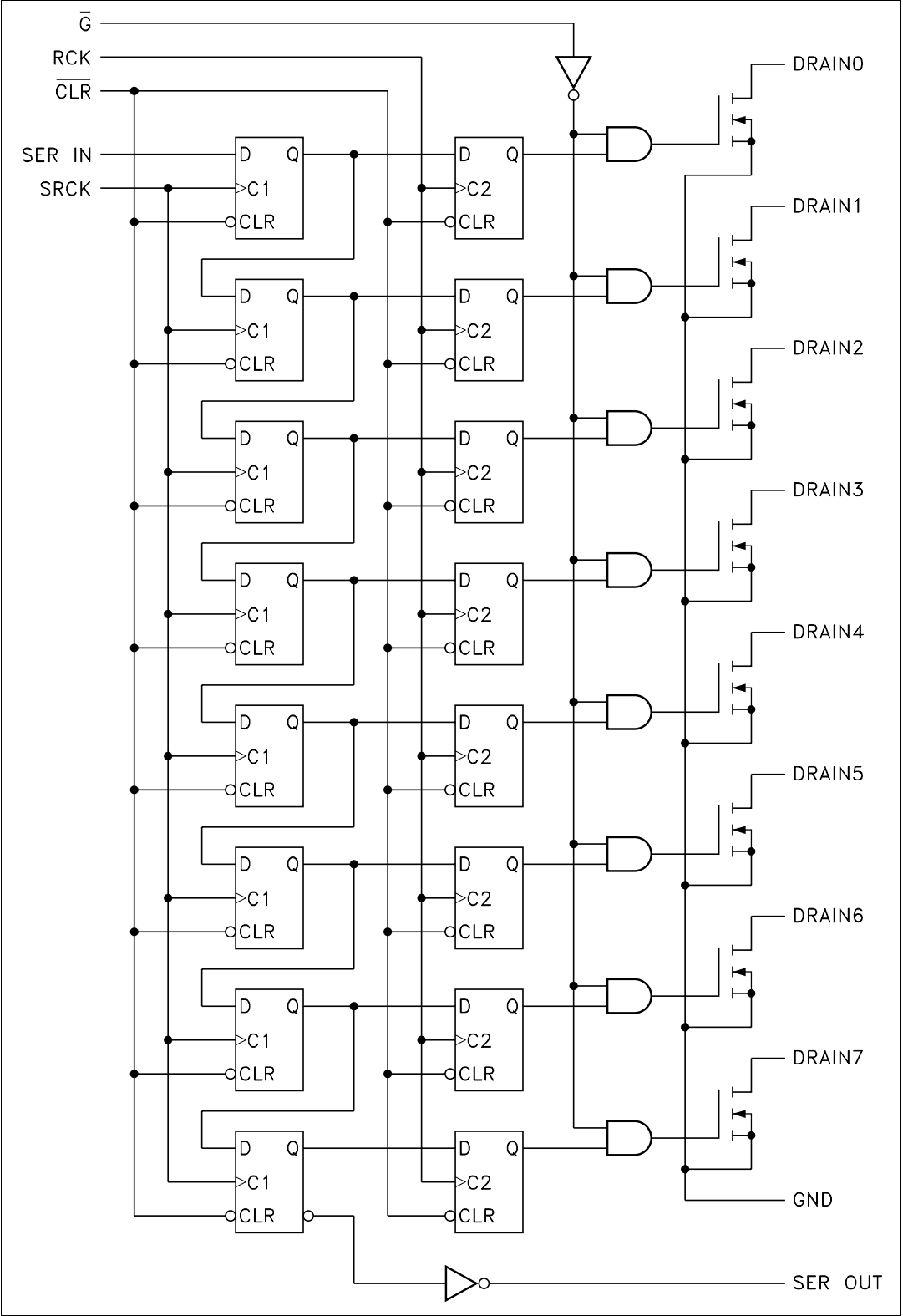
Figure 2. Logic diagram
