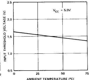
INPUT THRESHOLD VOLTAGE VS. AMBIENT TEMPERATURE
