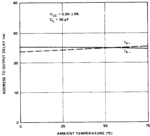
ADDRESS TO OUTPUT DELAY VS. AMBIENT TEMPERATURE
