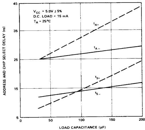
ADDRESS & CHIP SELECT TO OUTPUT DELAY VS. LOAD CAPACITANCE
