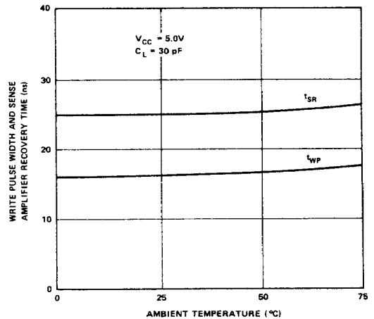
WRITE PULSE WIDTH & SENSE AMPLIFIER RECOVERY TIME VS. AMBIENT TEMPERATURE
