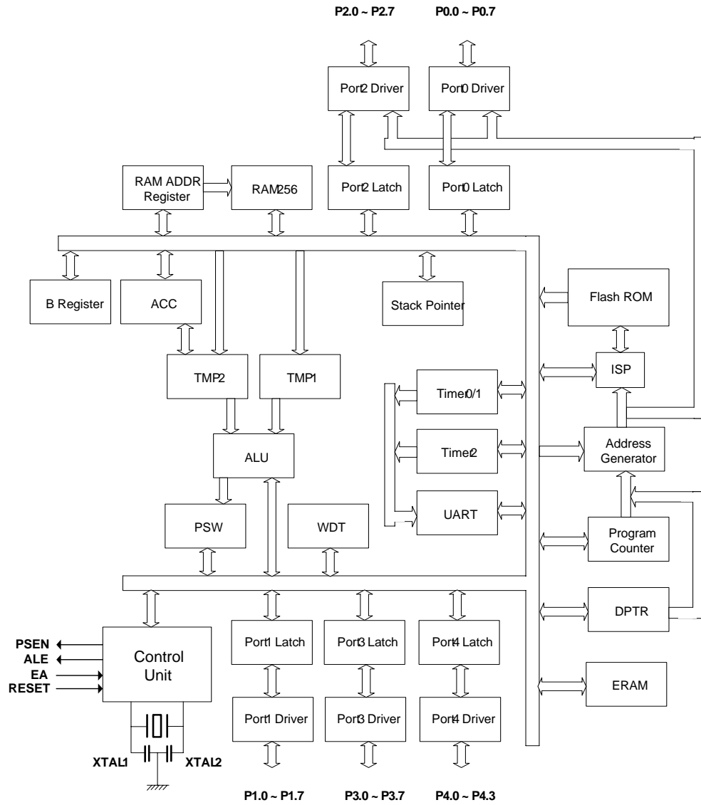
MPC89X52A Block Diagram
