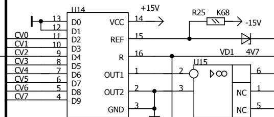
THREE CHANNEL ADC
